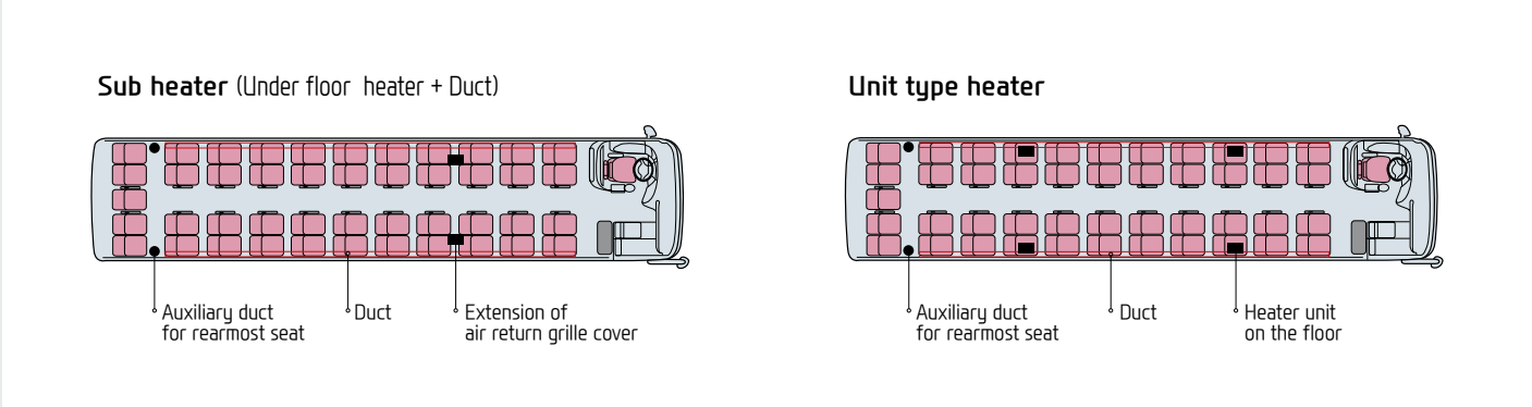
Air Control System
